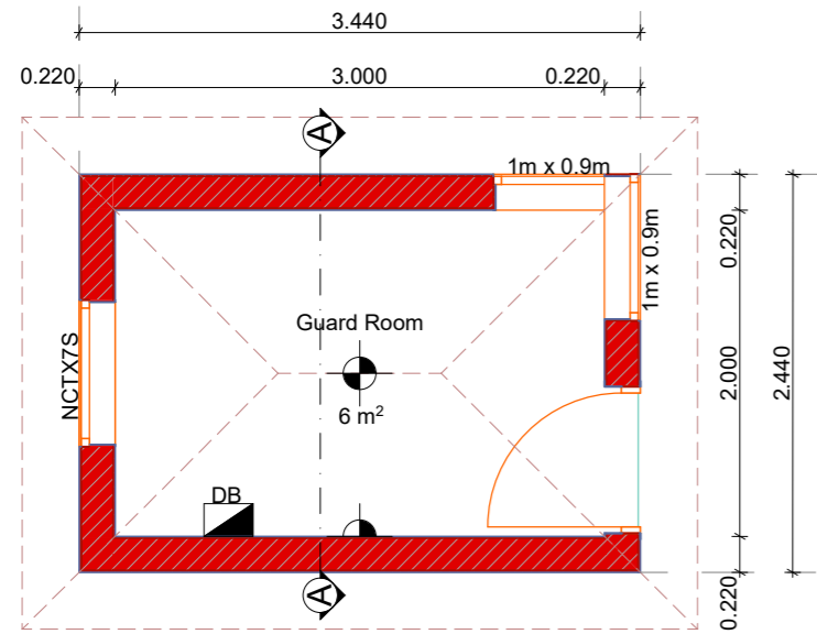
GROUND FLOOR PLAN SCALE 1:50
