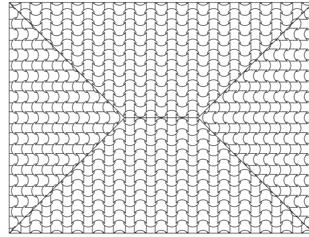
ROOFING PLAN SCALE 1:50
