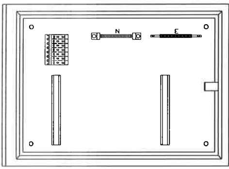
OPEN VIEW NO FACEPLATE
