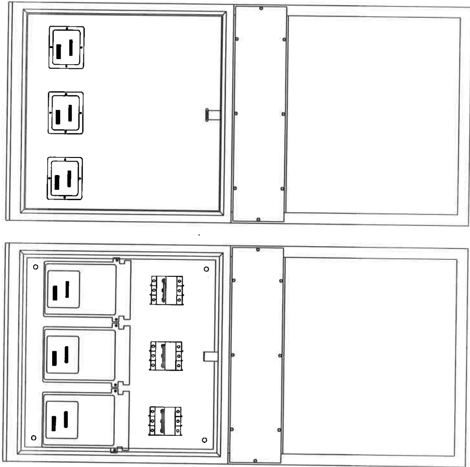
OPEN VIEW WITH FACEPLATE
